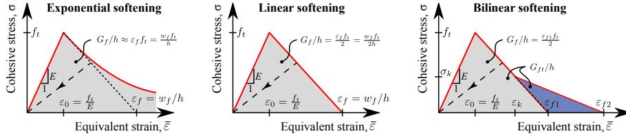
Figure 7: Implemented stress-strain diagrams for isotropic damage material. Fracturing strain \varepsilon_f and crack opening at zero stress w_f are interrelated through effective thickness h of the crack band. Note that exponential softening approach based on an exponential cohesive law is not exactly equivalent to the approach based on an exponential softening branch of the stress-strain diagram; see the detailed discussion of the damage laws.
