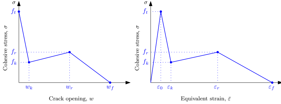
Figure 6: Trilinear softening diagram expressed in terms of the crack opening ( w ) and expressed in terms of strain.
