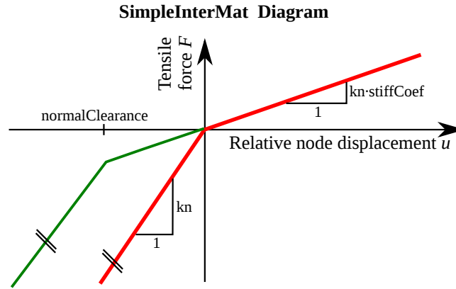
Figure 12: Working diagram of SimpleInterfaceMat.
