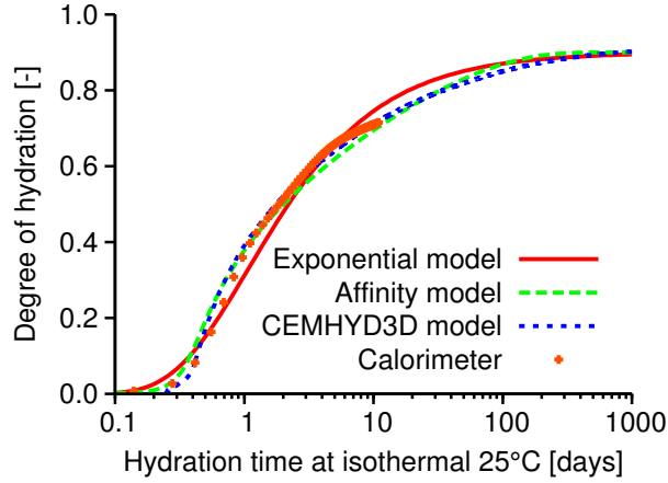
Figure 16: Performance of implemented hydration models: exponential model from Eq. (292), affinity model from Eq. (293), CEMHYD3D model from Sub-section 2.5.
