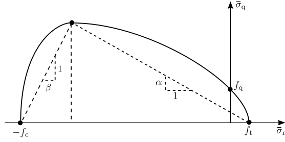
Figure 15: Latticeplastdam yield surface, which is composed of ellipse with a smooth transition.
