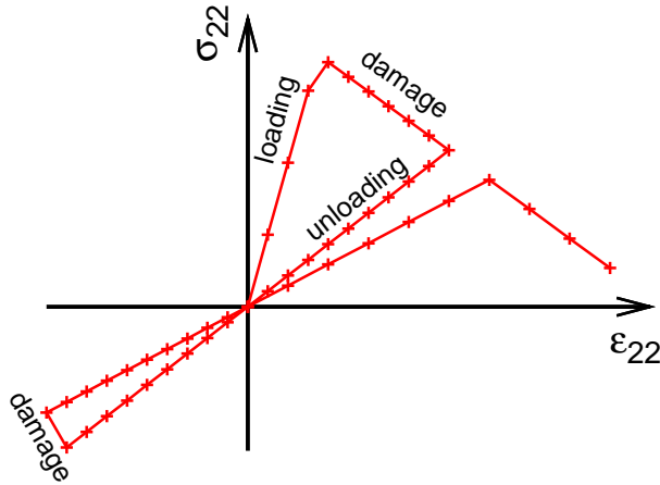
Figure 11: Typical loading/unloading material performance for homogenized stress and strain in the direction ‘2’. Note that one damage parameter is common for both tension and compression.
