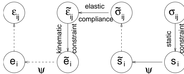
Figure 8: Structure of microplane-based anisotropic damage model
