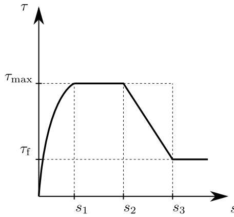
Figure 13: Bond stress ( \tau ) - reinforcement slip ( s ) diagram for BondCEB model.
