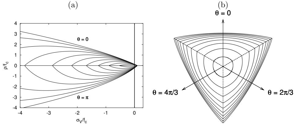
Figure 9: Evolution of the yield surface during hardening: a) meridional section, b) deviatoric section for a constant volumetric effective stress of \bar{\sigma}_V = -\bar{f}_c/3
